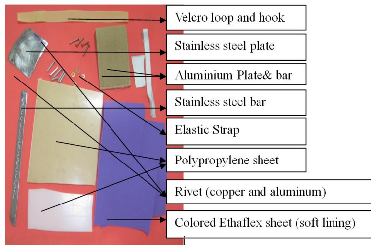
FIGURE 1: Components of the Modified dual axis knee brace
